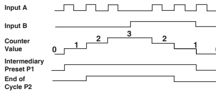
UP/DOWN Counter with Preset=1 (Intermediary) & Preset= 2 (End of Cycle)
