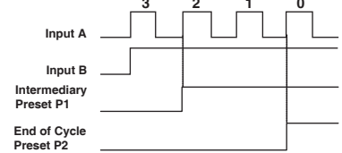
Down Counter With Preset 2 ( Intermediary ) & 4 ( End Of Cycle)
