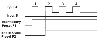
UP Counter With Preset=1 (Intermediary) and 2 (End of Cycle)
