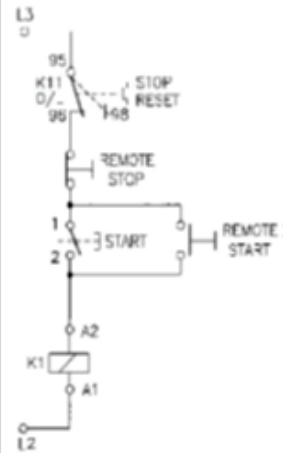
CONTROL CIRCUIT (FOR REMOTE CONTROL)
