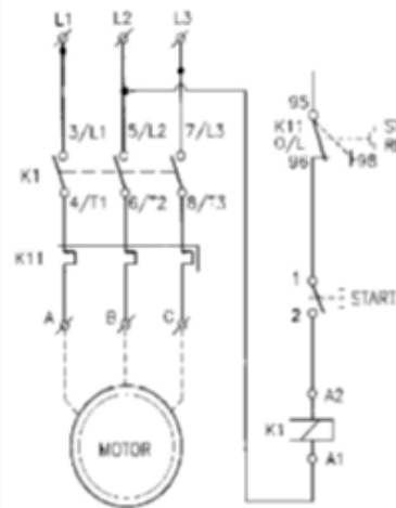
WIRING DIAGRAM
