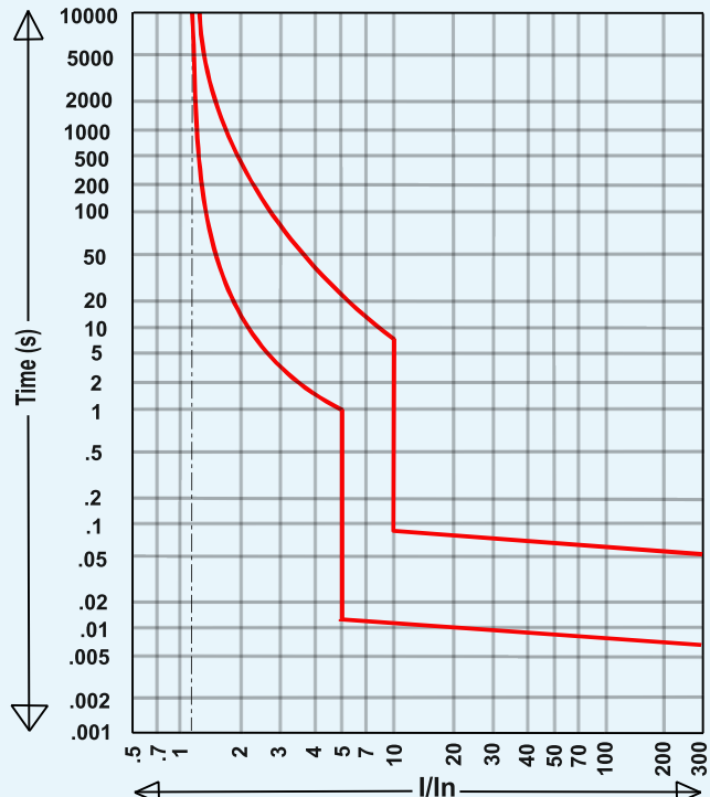
'C' Characteristics
