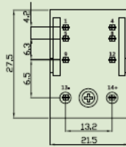
WIRING LAYOUT (BOTTOM VIEW)
