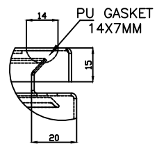
DETAIL OF "A"
