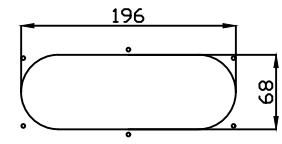
CABLE ENTRY PLATE CUTOUT
