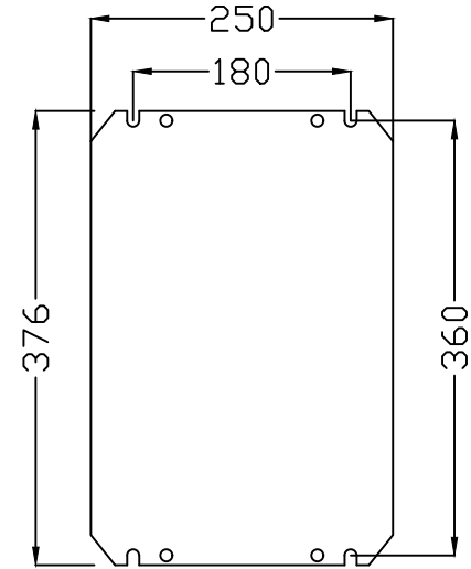
MOUNTING PLATE
