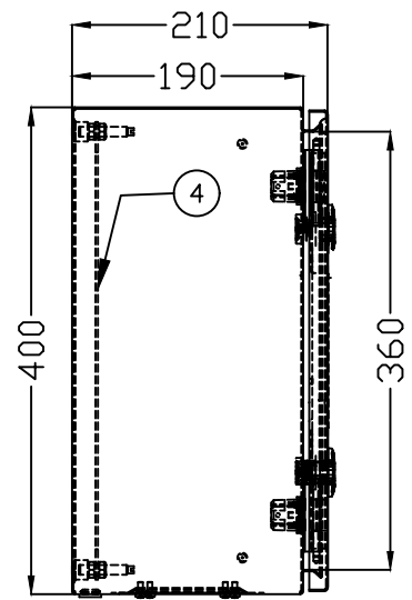
LHS VIEW
