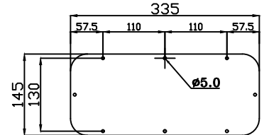
CABLE ENTRY PLATE
