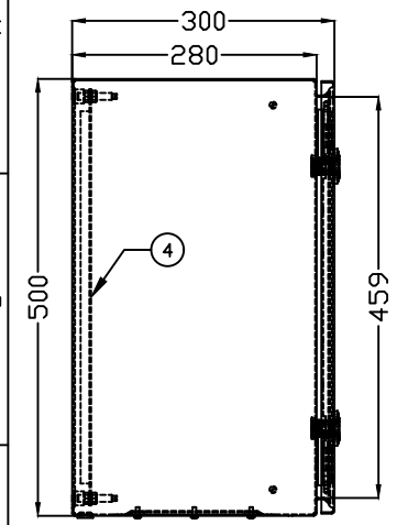
LHS VIEW
