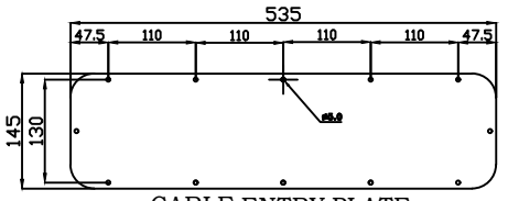
CABLE ENTRY PLATE
