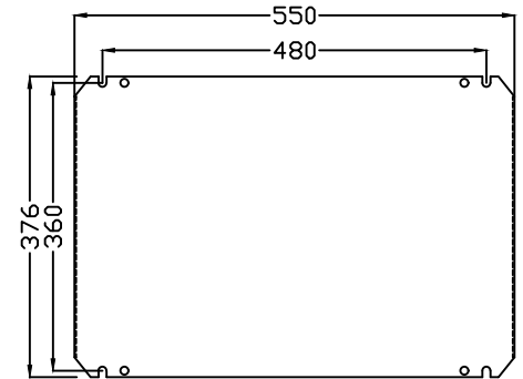
MOUNTING PLATE
