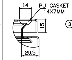
DETAIL OF "A"
