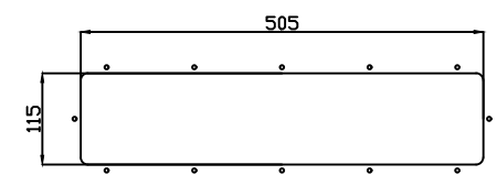
CABLE ENTRY CUTOUT
