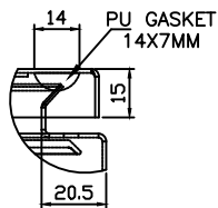
DETAIL OF "A"
