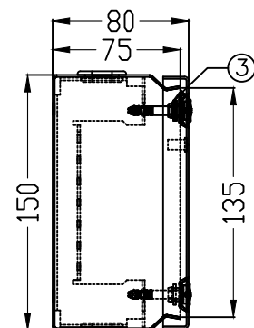
LHS VIEW
