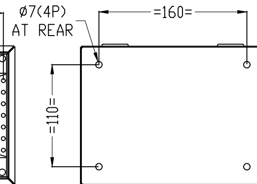
REAR VIEW
