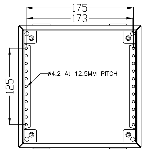
FRONT VIEW WITHOUT FRONT COVER
