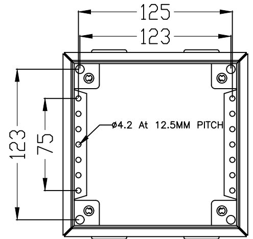
FRONT VIEW WITHOUT FRONT COVER
