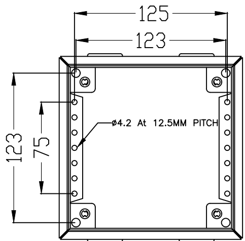
FRONT VIEW WITHOUT FRONT COVER
