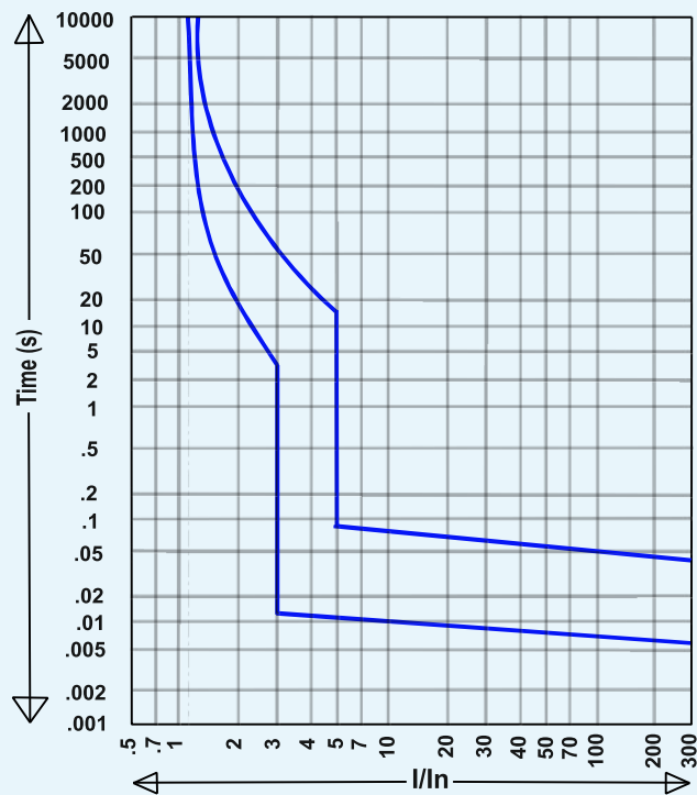
‘B’ Characteristics
