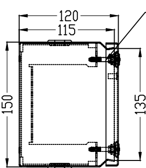
LHS VIEW
