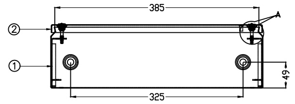
BOTTOM VIEW
