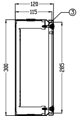
LHS VIEW
