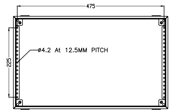
FRONT VIEW WITHOUT FRONT COVER
