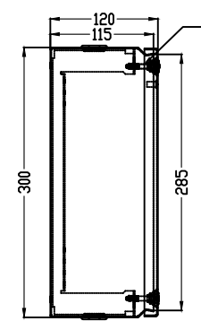
LHS VIEW
