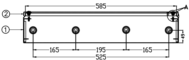
BOTTOM VIEW
