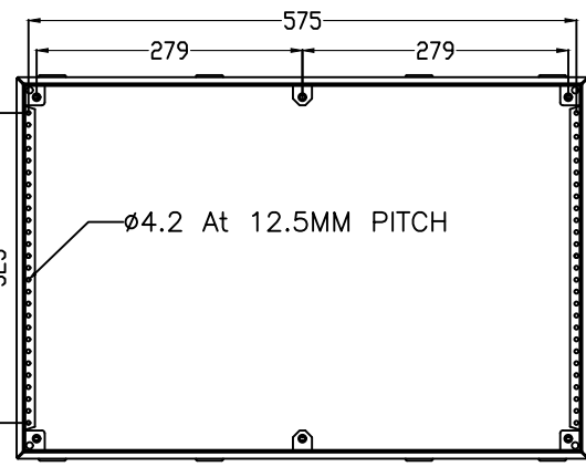
FRONT VIEW WITHOUT FRONT COVER
