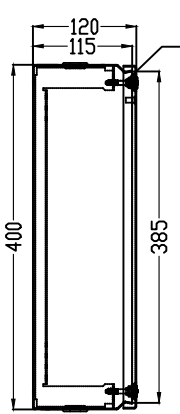
LHS VIEW
